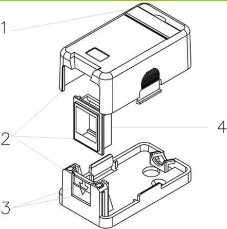
1-port w/ shutter (37 × 65 × 30 mm)
