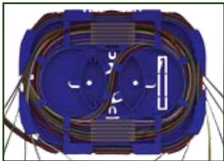
Internal Fibre Management Channels and cross over radius protection
