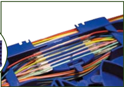
Hinged style holder for heat shrink splice holder
