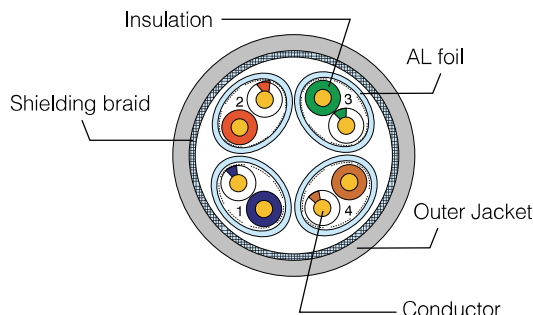
Cross section
