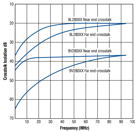
Figure 3: Balanced Crosstalk
