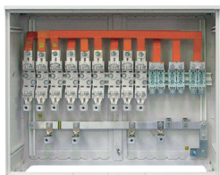
SR508/NVW+P2
